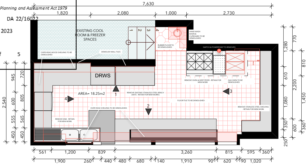
Demolition Floor Plan
